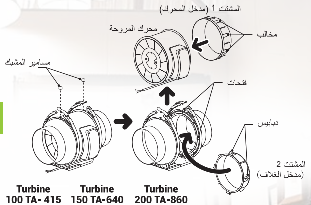
Turbine 150 TA-640
